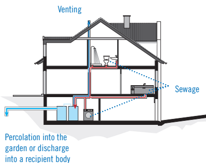
Illustration 1: Complete solution for single and share occupancy houses with car a cellar
