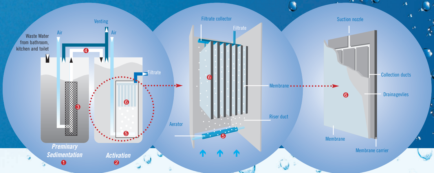
Illustration 4: Functional diagram of the membrane module
